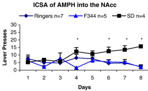
Fig. 2. Comparison of SD and F344 AMPH self-administering groups revealed a significant main effect of strain ( F_{(1,7)}=14.029 ; p=0.007 ) and a significant interaction between strains and days ( p<0.001 ). Student Newman–Keuls posthoc analysis showed significantly more lever pressing for AMPH by SD than by F344 rats on days 4, 6, 7, and 8 ( *p<0.05 ). ICSA=intracranial self-administration, AMPH=amphetamine, NAcc=nucleus accumbens, SD=Sprague–Dawley, F344=Fischer 344.
